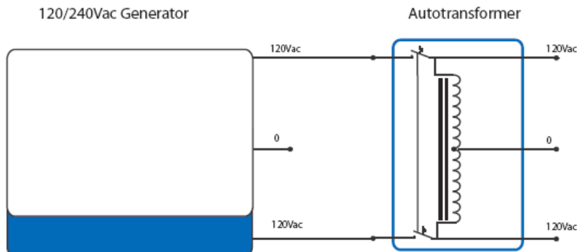
Stacked inverter balancing (Ground relay of autotransformer should be used)
